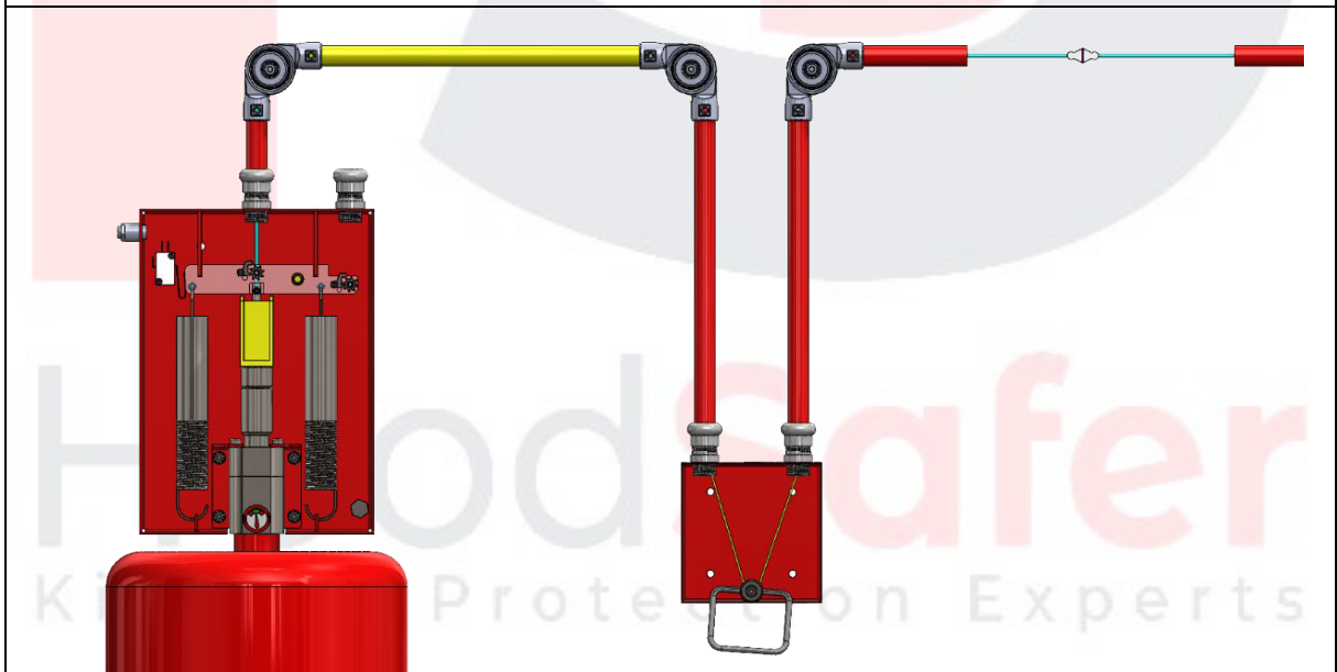
MID-LINE Installation of MANUAL PULL STATION (P300)
