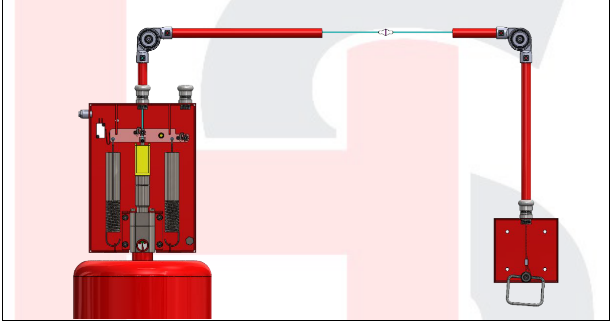
END OF LINE Installation of MANUAL PULL STATION (P300)
